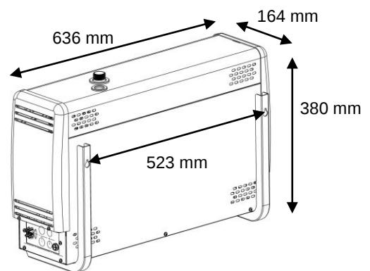
Wandmontage stoomgenerator
