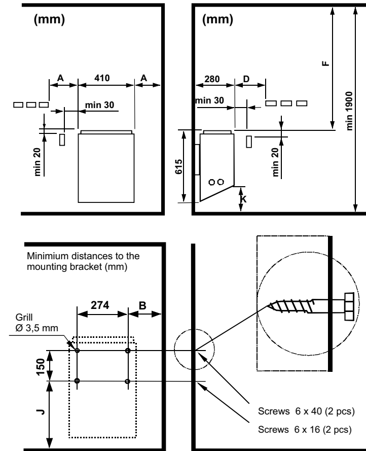
Image 2. Safety clearances
