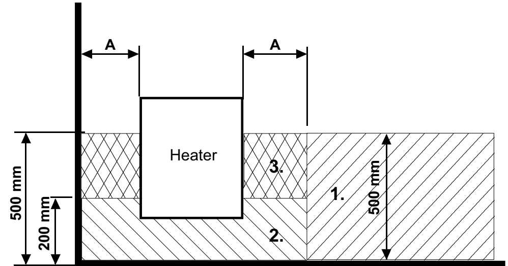
Image 3. Locating the connection box for connection cable in the sauna room
