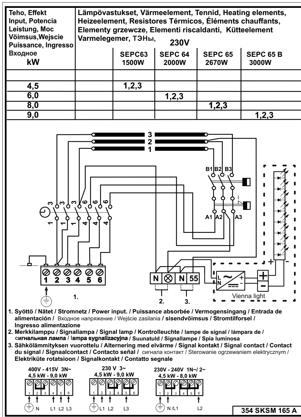
Image 4 Wiring diagram
