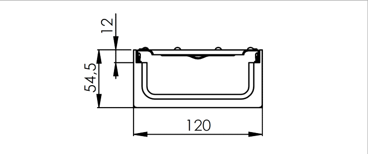
Grating details
