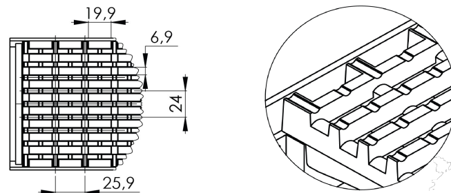
Grating details
