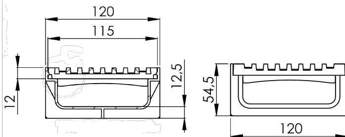
Cross-Section
